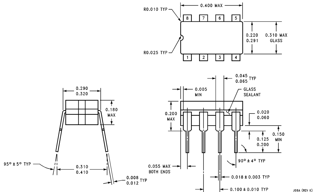
Ceramic Dual-In-Line Package (J) Order Number LM4250J-MIL NS Package Number J08A
