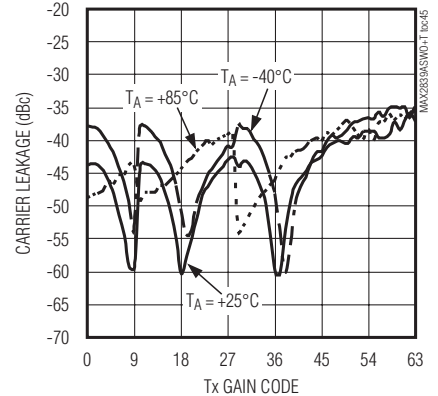
Tx CARRIER LEAKAGE vs. GAIN SETTING
