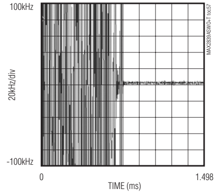
CHANNEL-SWITCHING FREQUENCY SETTLING (2.3GHz TO 2.7GHz, AUTOMATIC VCO SUB-BAND SELECTION)
