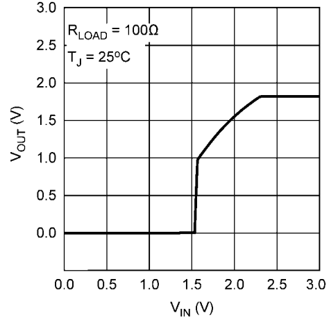
V OUT vs V IN , V OUT = 1.80V
