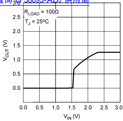
V OUT vs V IN , V OUT = 1.25V 查询"LP38693-ADJ"供应商
