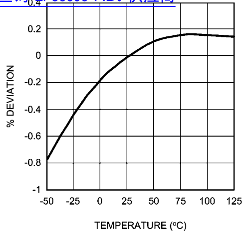
V REF vs Temperature 查询"LP38693-ADJ"供应商
