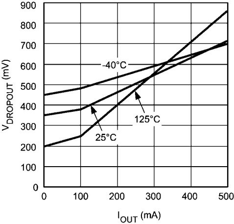
Dropout Voltage vs I_{OUT} ( V_{SUP} = 1.8V )
