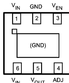
6-Lead LLP, Bottom View LP38693SD-ADJ
