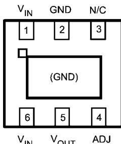
6-Lead LLP, Bottom View LP38691SD-ADJ
