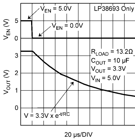
V OUT vs V EN , OFF (LP38693 Only)
