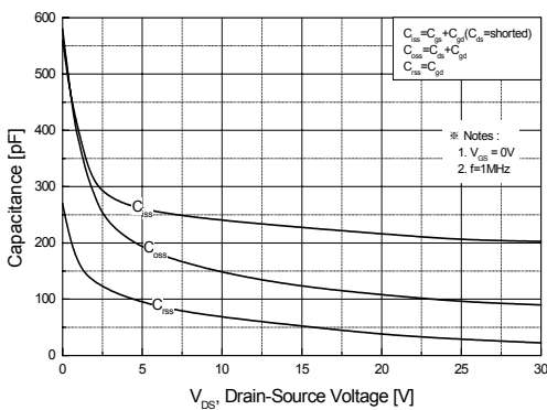
Fig 5. Capacitance Characteristics
