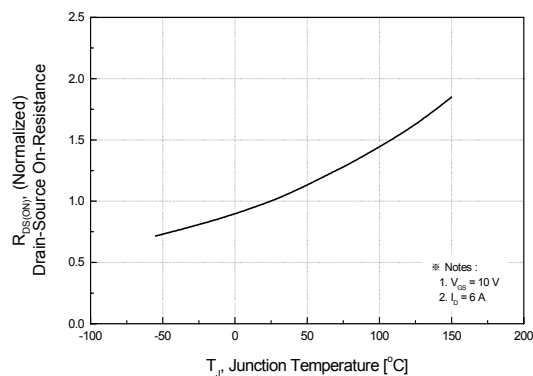
Fig 8. On-Resistance Variation vs. Junction Temperature
