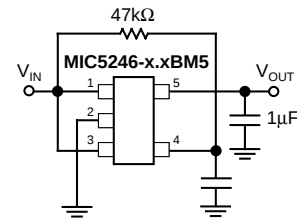
Figure 1. Low-Noise Fixed Voltage Application
