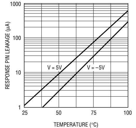
Response Pin Leakage vs Temperature (Device Off)
