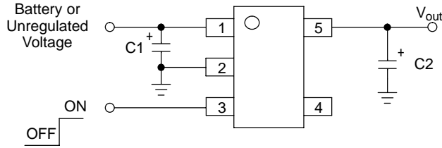
Figure 27. Typical Application Circuit
