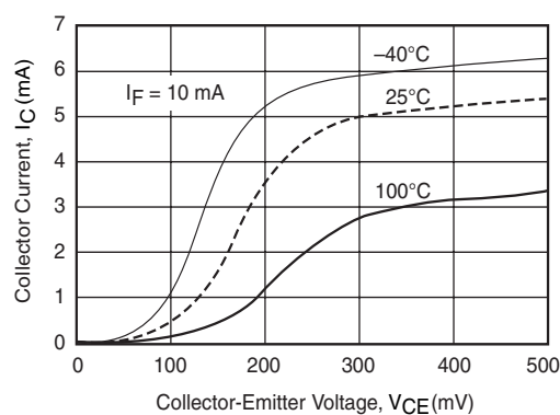
Fig. 4 Collector Current vs. Collector Emitter Voltage
