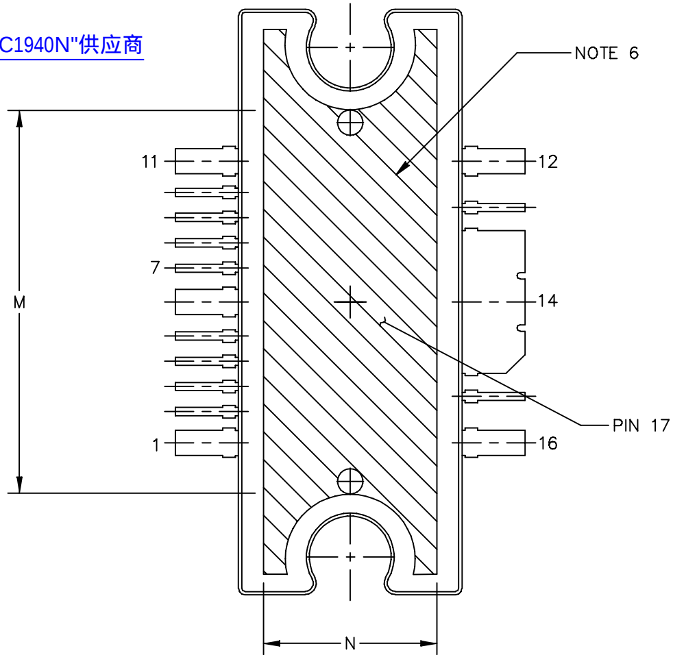
VIEW Y-Y
