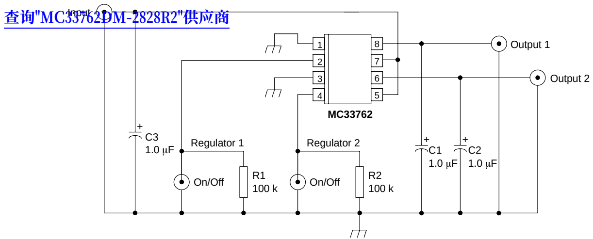
Figure 7. A Typical Application Schematic
