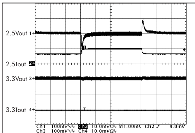
Figure 15: Output voltage response to step-change in Iout1 (50%-75%-50% of Imax; dI/dt = 0.1A/μs). Load cap: 15μF, 300 mΩ ESR tantalum & 1μF ceramic. Vout (100mV/div), Iout (10A/div). Ch1: Vout1; Ch2 Iout1; Ch 3: Vout2; Ch 4 Iout2
