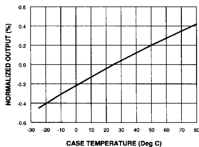
OUTPUT VOLTAGE Vs CASE TEMPERATURE
