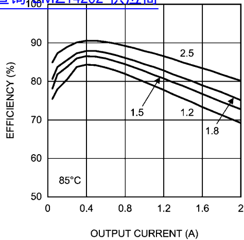
Efficiency 6V Input @ 85°C 查询"LMZ14202"供应商
