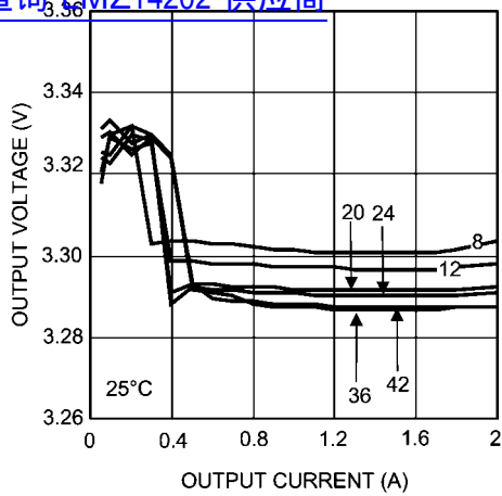
Line and Load Regulation @ 25°C 查询"LMZ14202"供应商
