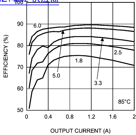
Efficiency 24V Input @ 85°C 查询"LMZ14202"供应商
