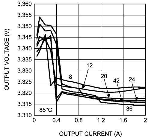
Line and Load Regulation @ 85°C
