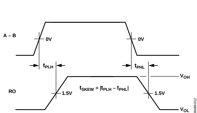
Figure 17. Receiver Propagation Delay
