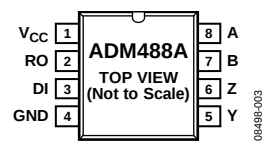
Figure 3. ADM488A Pin Configuration
