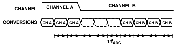
Figure 37. Sinc 3 Channel Change
