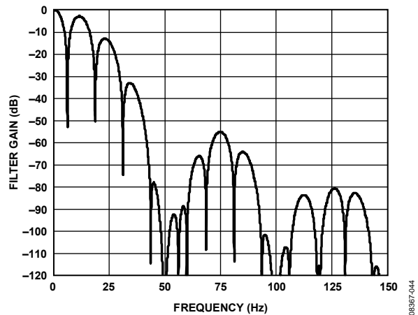
Figure 48. Sinc^4 Filter Response ( FS[9:0] = 96 , Chop Enabled, REJ60 = 1 )
