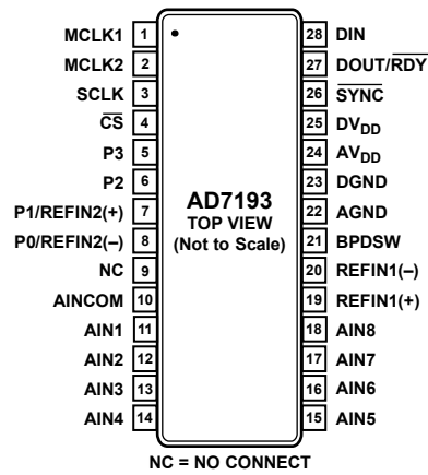
Figure 5. 28-lead TSSOP Pin Configuration
