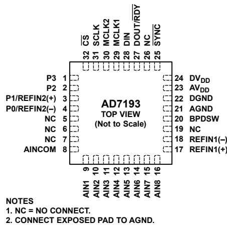
Figure 6. 32-Lead LFCSP Pin Configuration
