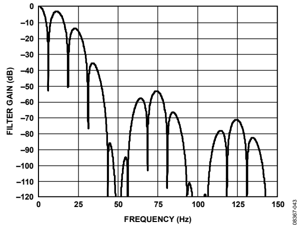
Figure 47. Sinc^4 Filter Response ( FS[9:0] = 96 , Chop Enabled)
