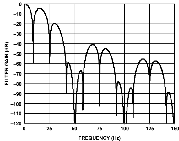
Figure 52. Sinc 3 Filter Response ( FS[9:0] = 96 , Chop Enabled)
