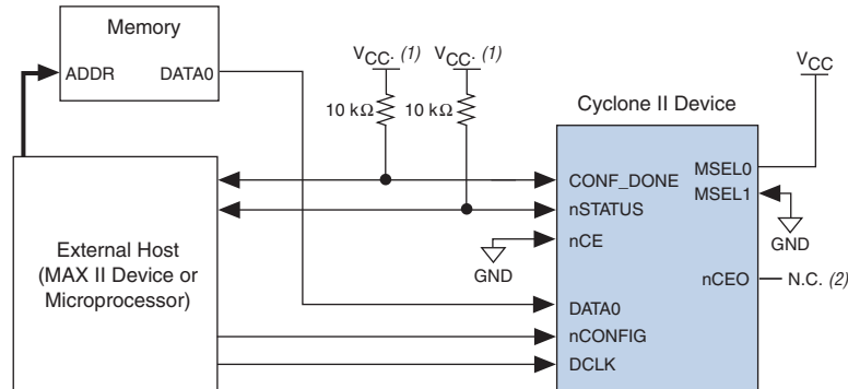
Figure 13–9. Single Device PS Configuration Using an External Host
