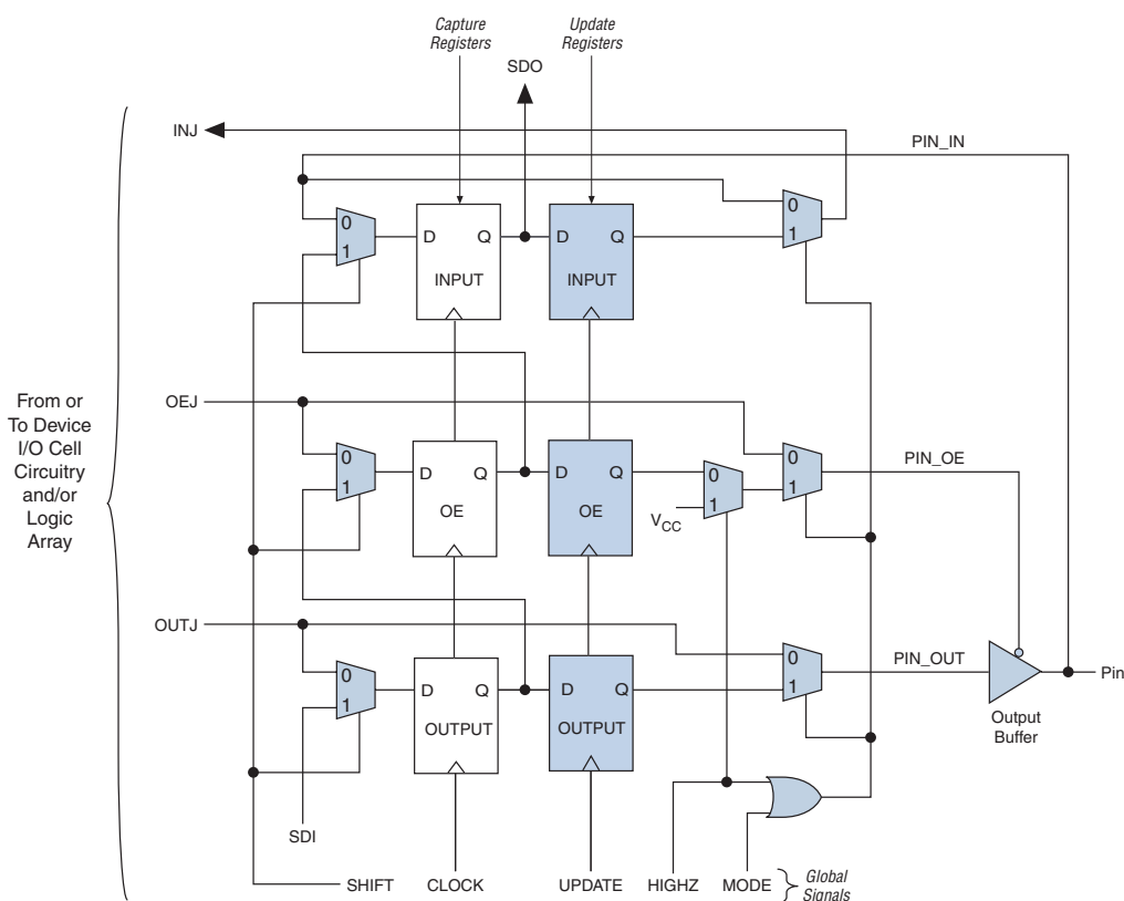
Figure 14–4. Cyclone II Device's User I/O BSC with IEEE Std. 1149.1 BST Circuitry
