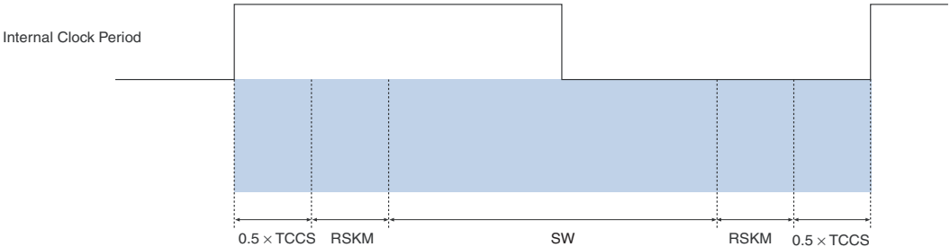
Figure 5–4. High-Speed I/O Timing Budget Note (1)
