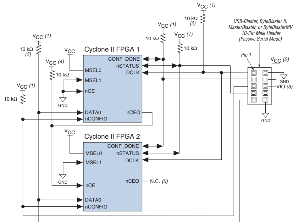
Figure 13–20. Multiple Device PS Configuration Using a USB-Blaster, MasterBlaster, ByteBlaster II or ByteBlasterMV Cable
