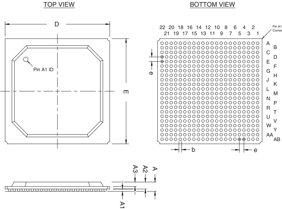
Figure 15–5. 484-Pin FineLine BGA Package Outline
