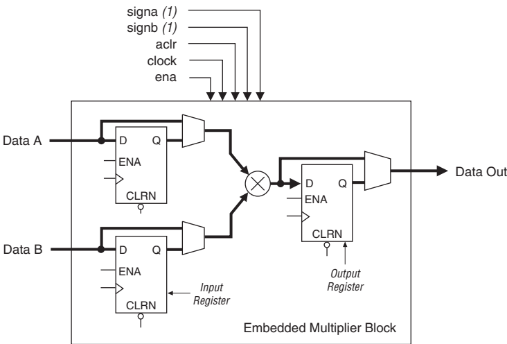
Figure 2-18. Multiplier Block Architecture
