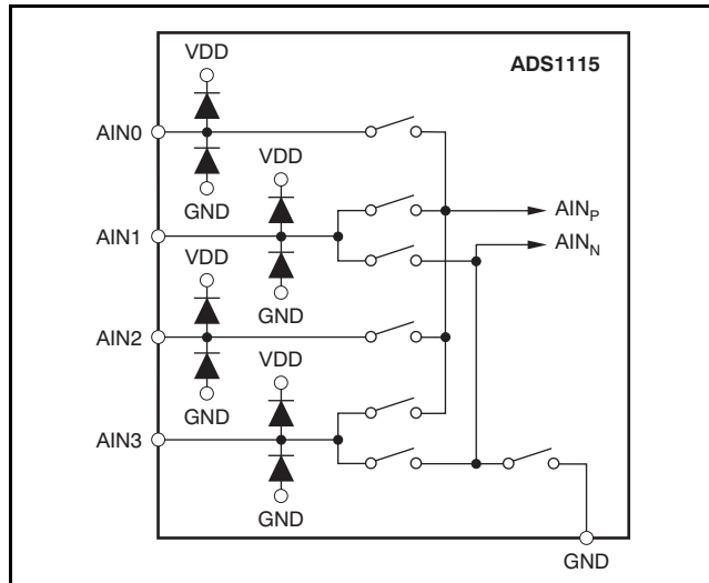
Figure 24. ADS1115 MUX
