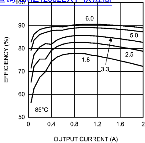
Efficiency 20V Input @ 85°C 查询"LMZ12002EXT"供应商
