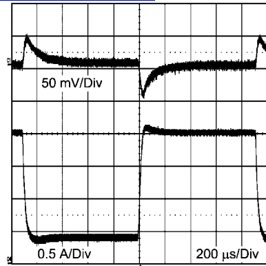
Transient Response V_{IN} = 3.3V to 2A Step
