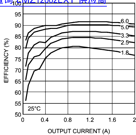
Efficiency 20V Input @ 25°C 查询LMZ12002EXT"供应商"
