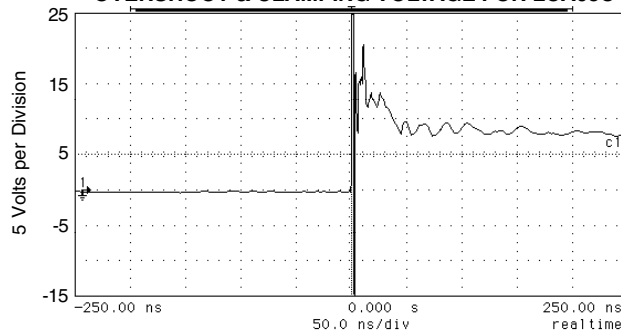
FIGURE 4 OVERSHOOT & CLAMPING VOLTAGE FOR LCA05C
