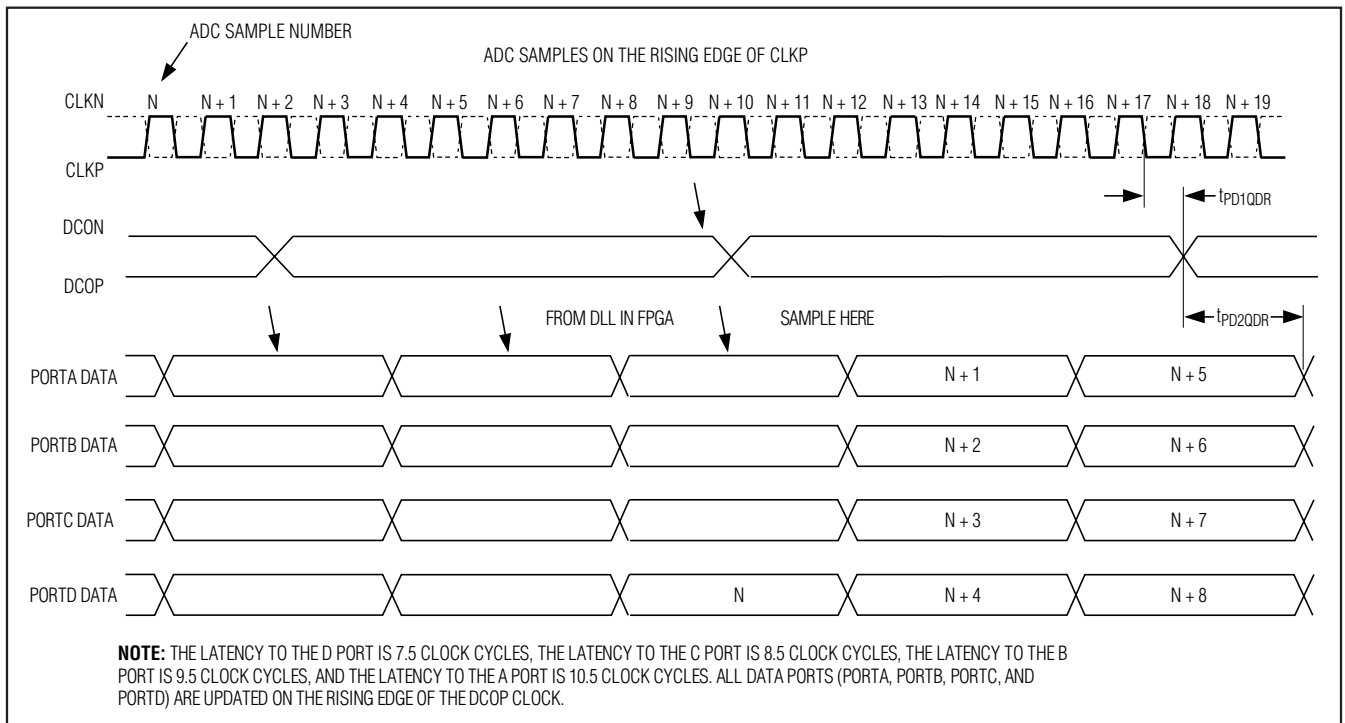
Figure 8. Timing Diagram for QDR Mode, f_{CLK}/16 Mode
