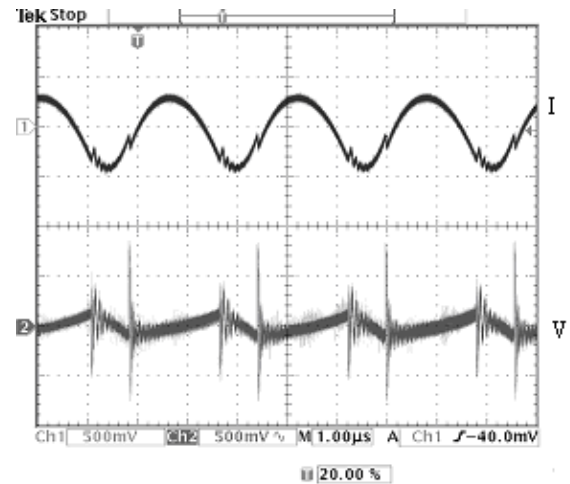
Photo 8: Input Reflected Ripple Voltage and Ripple Current V_{in}=24V , I_{out} = 10A
