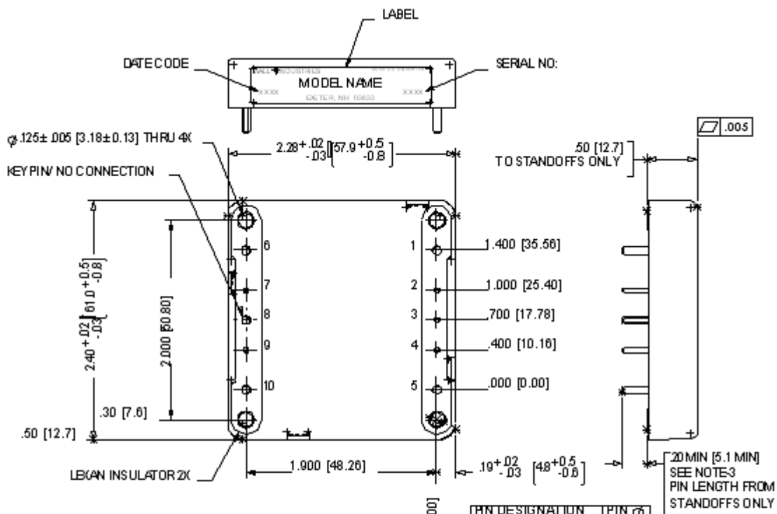
Figure 1: Mechanical Dimensions
