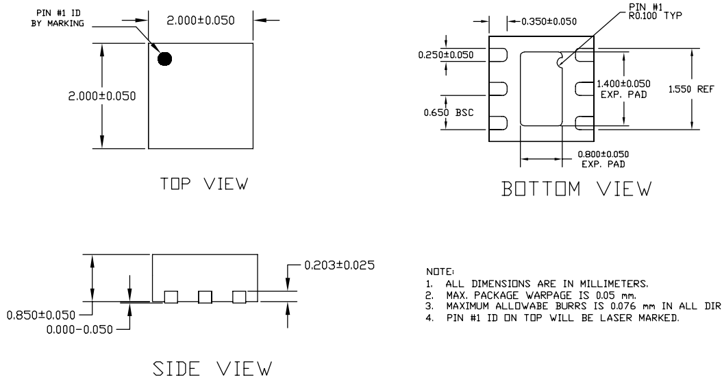
6-Pin 2mm x 2mm MLF ® (ML)
