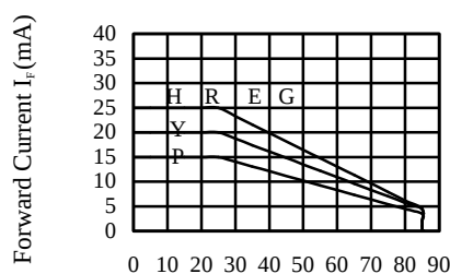
FIG.3 ALLOWABLE DC CURRENT VS. AMBIENT TEMPERATURE
