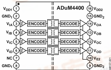
Figure 1. ADuM4400
