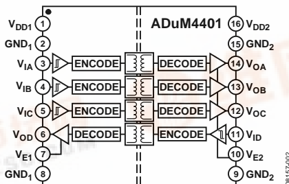
Figure 2. ADuM4401
