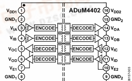
Figure 3. ADuM4402
