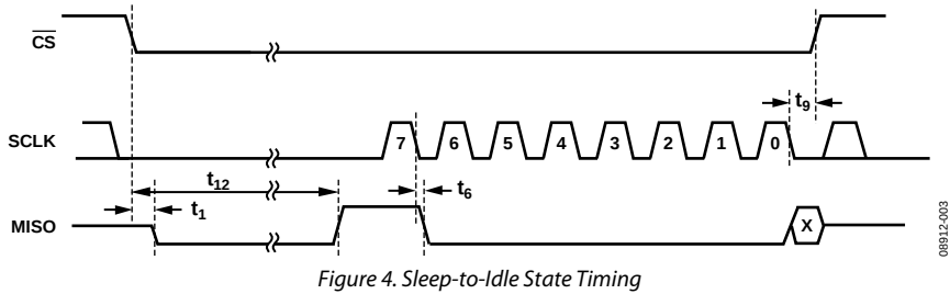
Figure 4. Sleep-to-Idle State Timing
