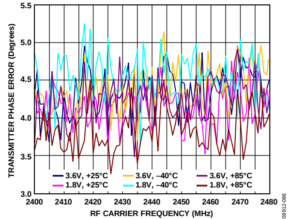
Figure 60. 500 kbps GFSK ( f_{DEV} = \pm 250 kHz) Mode Transmitter Phase Error vs. Temperature, VDD_BAT, and Channels, 1 MHz Channel Step, Output Power = 3 dBm
