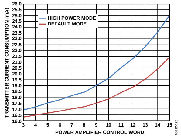
Figure 67. Transmitter Current Consumption vs. Control Word, for Default and High Power Modes, f_{\text{CHANNEL}} = 2.45 \text{ GHz} , V_{\text{DD\_BAT}} = 3.6 \text{ V} , Temperature = 25^\circ\text{C}
