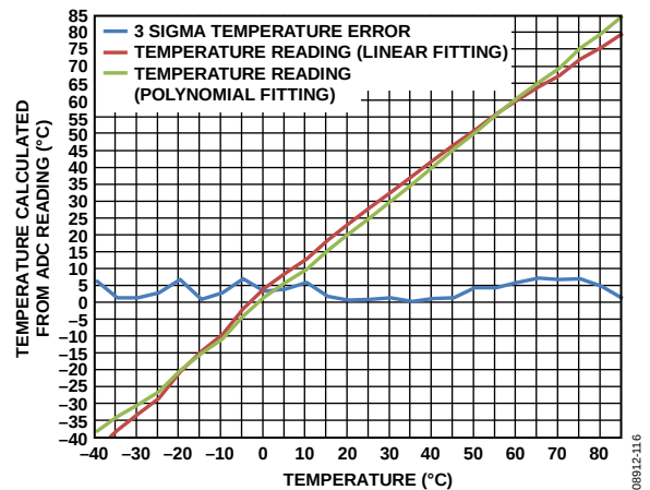
Figure 68. Temperature Sensor Performance (Average of 1000 ADC Readbacks) and 3-\Sigma Error vs. Temperature, V_{\text{DD\_BAT}} = 3.6 \text{ V}
