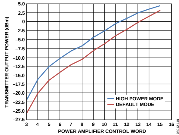
Figure 66. Transmitter Output Power vs. Control Word for Default and High Power Modes, f_{\text{CHANNEL}} = 2.45 \text{ GHz} , V_{\text{DD\_BAT}} = 3.6 \text{ V} , Temperature = 25^\circ\text{C} , RF Carrier Frequency, Temperature, and V_{\text{DD\_BAT}} (A discrete matching network and a harmonic filter are used as per the ADF7242 reference design.)
