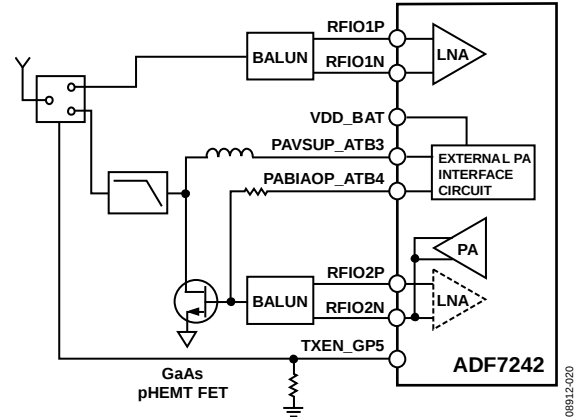
Figure 81. Typical External PA Applications Circuit
