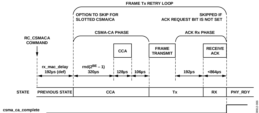
Figure 90. Automatic CSMA/CA Transmit Operation (with CCA)
