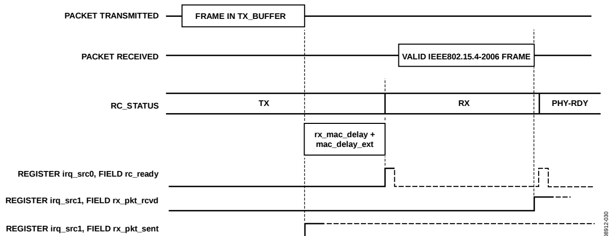
Figure 88. IEEE 802.15.4-2006 Auto TX-to-RX Turnaround Mode
