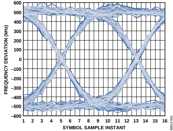
Figure 55. 2 Mbps GFSK ( f_{DEV} = \pm 500 kHz) Mode Transmitter Eye Diagram, f_{CHANNEL} = 2.45 GHz, Output Power = 3 dBm, VDD_BAT = 3.6 V, Temperature = 25°C
