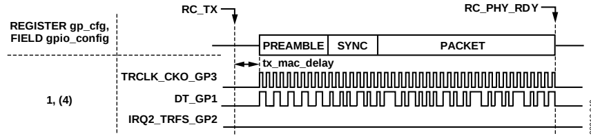
Figure 97. SPORT Operation in GFSK/FSK TX State
