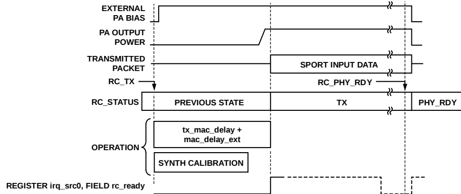
Figure 79. TX Timing and Control (GFSK/FSK SPORT Mode)
