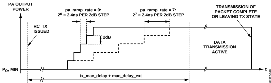
Figure 80. PA Ramping Profile
