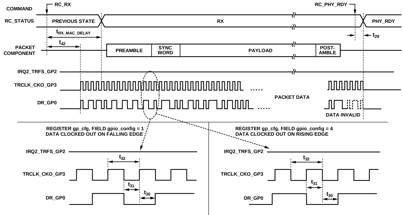
Figure 10. GFSK/FSK RX SPORT Mode: CLK and Data Pins Active in RX, Without Gating by Frame Detection
