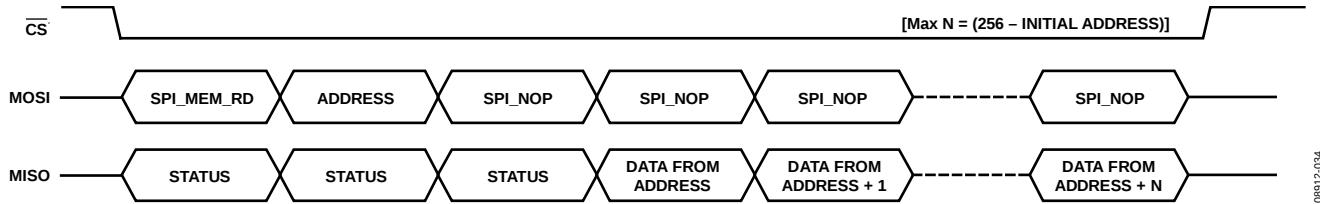
Figure 112. Memory (Register or Packet RAM) Block Read
