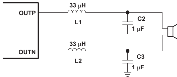
Figure 41. Typical LC Output Filter, Cutoff Frequency of 27 kHz, Speaker Impedance = 8 \Omega
