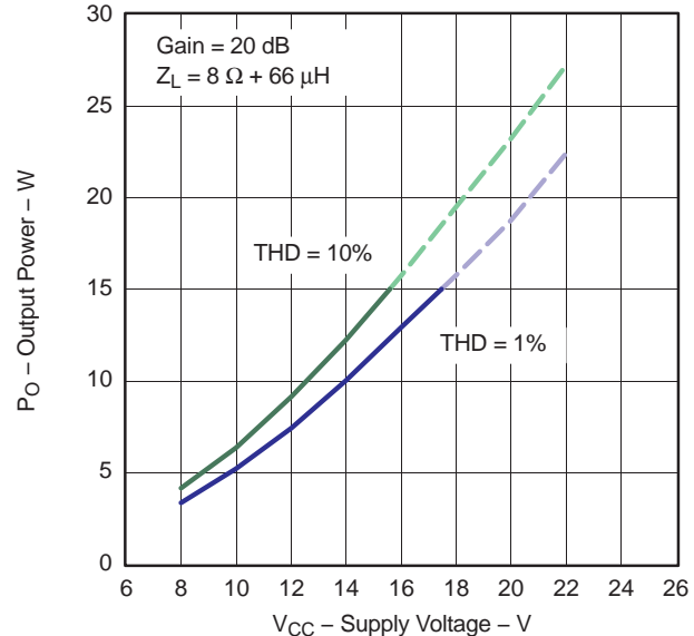
OUTPUT POWER vs SUPPLY VOLTAGE (BTL)
