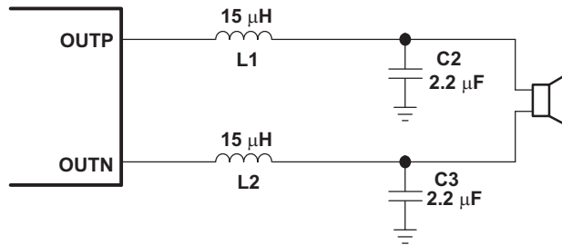
Figure 42. Typical LC Output Filter, Cutoff Frequency of 27 kHz, Speaker Impedance = 4 \Omega
