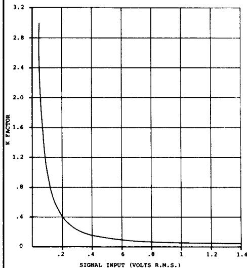
GRAPH 5 GRAPH SHOWING K FACTOR VS SIGNAL INPUT AMPLITUDE.
