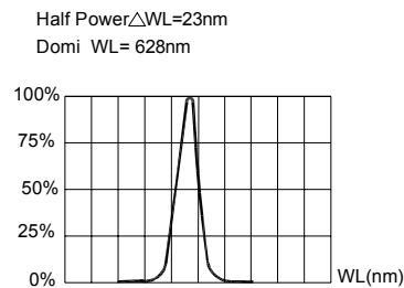
FIG.4 RELATIVE INTENSITY VS. WAVE LENGTH.
