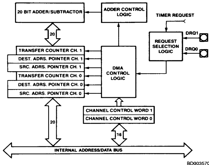
Figure 16. DMA Unit Block Diagram
