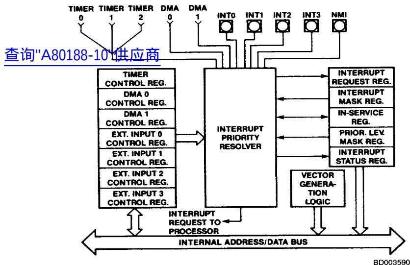
Figure 21. Interrupt Controller Block Diagram
