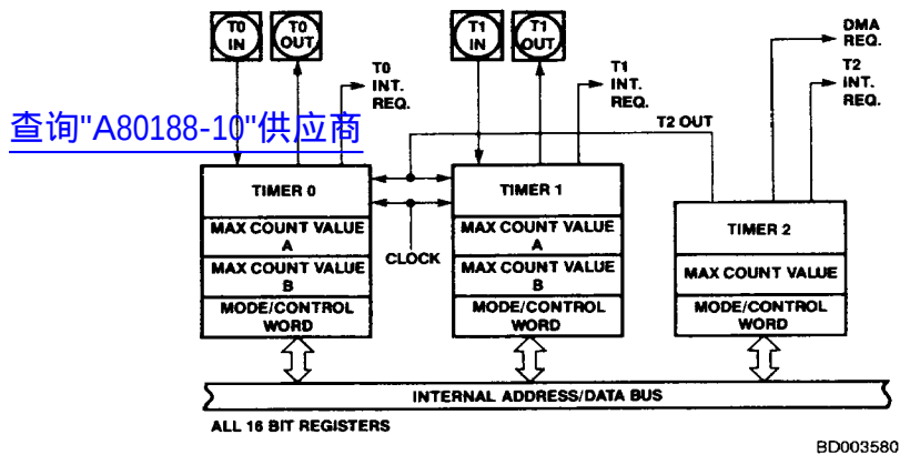
Figure 19. Timer Block Diagram
