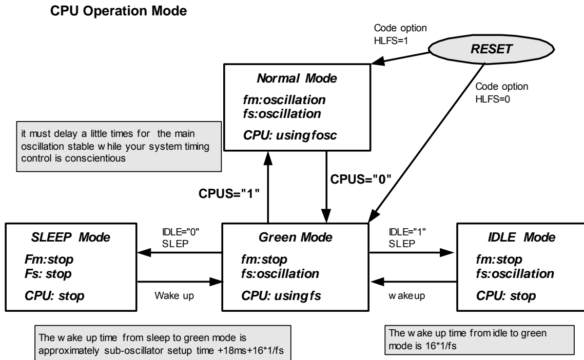
Fig. 6-3 CPU Operation Mode
