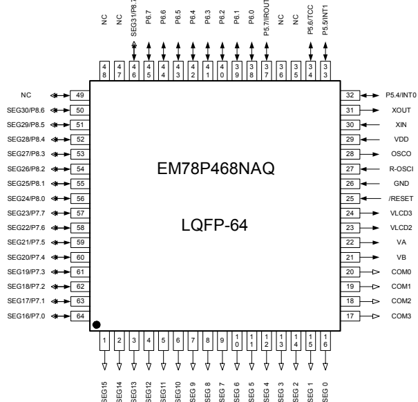
Fig. 3-2 64-pin LQFP
