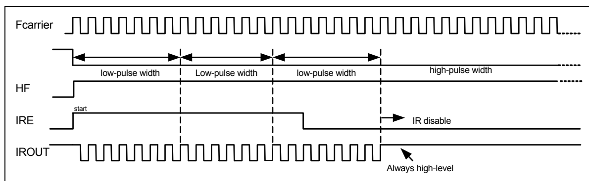
Fig. 6-25 LGP=1, IROUT Pin Output Waveform
