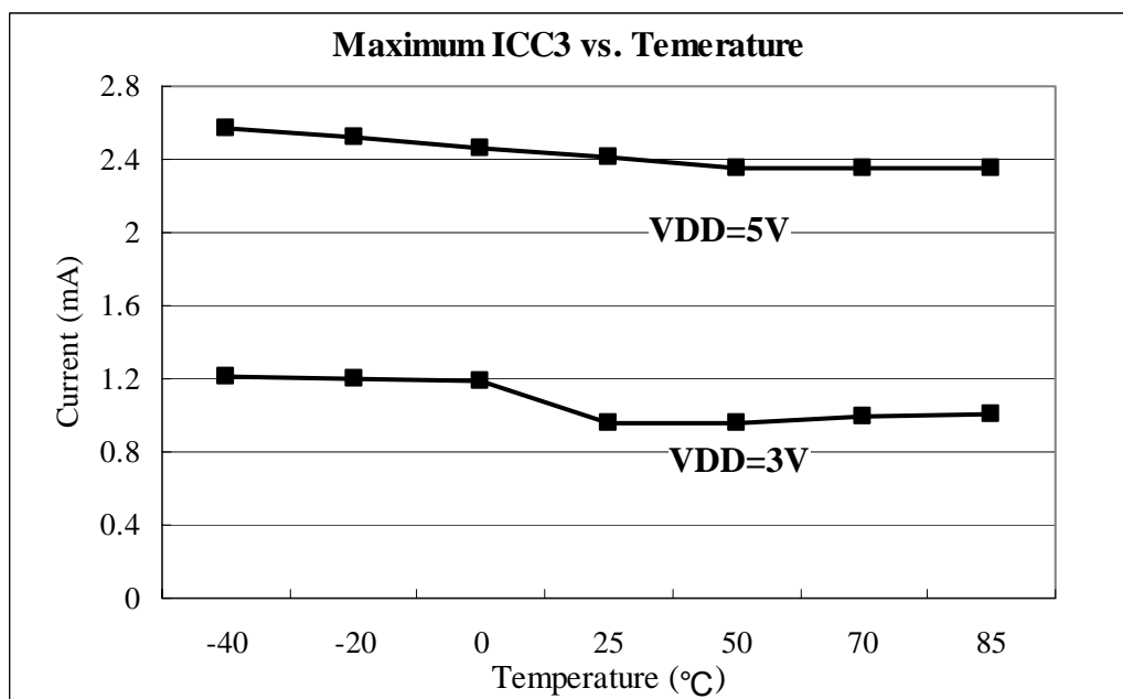
Fig. 8-15 Maximum Power Consumption on Normal Mode Operation (Fm=4MHz)
