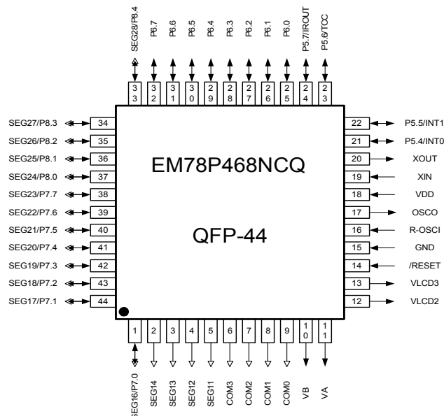
Fig. 3-4 44-pin QFP
