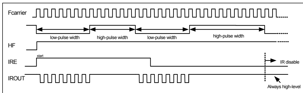
Fig. 6-23 LGP=0, IROUT Pin Output Waveform
