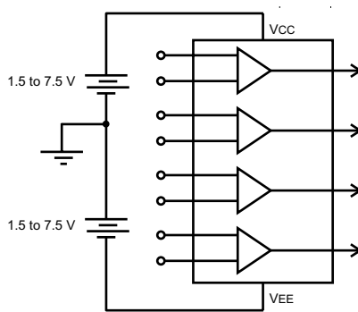
Split Supply
