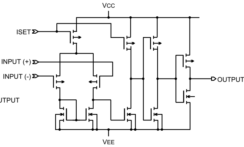
Comparator
