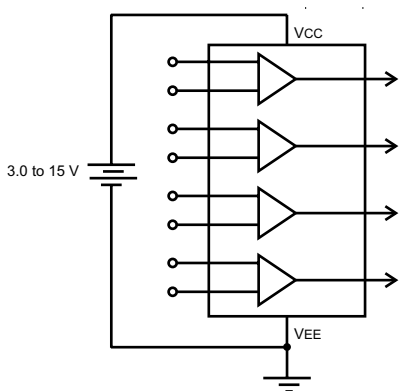
Single Supply
