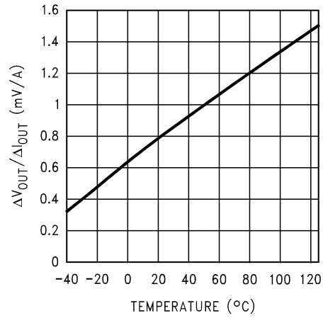
DC Load Regulation
