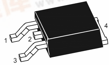
1. Base 2. Collector 3. Emitter 4. Collector TO-252 Plastic Package
