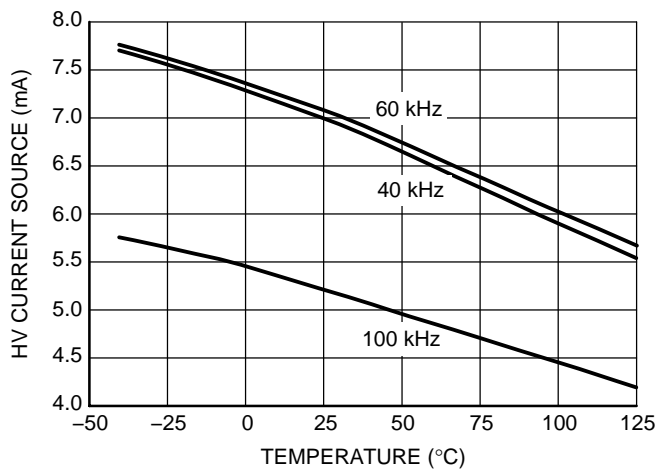
Figure 7. HV Current Source at V_{CC} = 10\text{ V} versus Temperature
