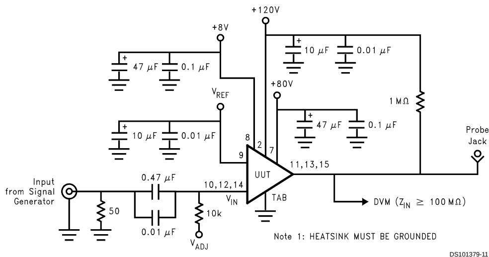
FIGURE 11. Test Circuit (One Channel)
