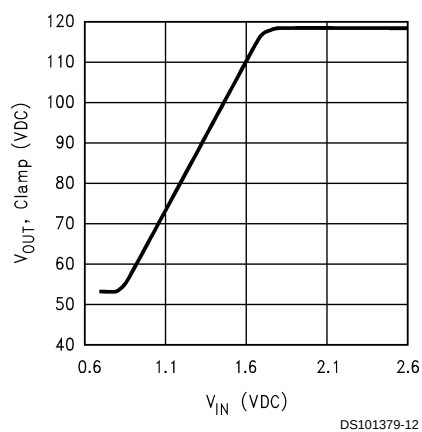
FIGURE 12. Clamp Circuit V_O vs. V_{IN}
