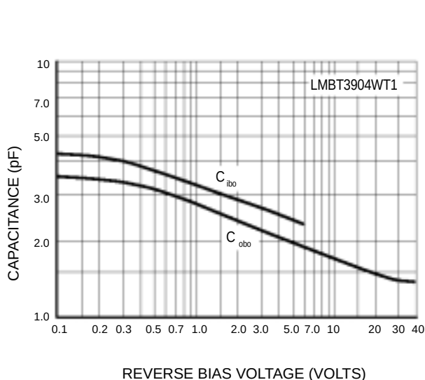
REVERSE BIAS VOLTAGE (VOLTS) Figure 3. Capacitance
