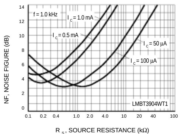
Figure 10. Noise Figure
