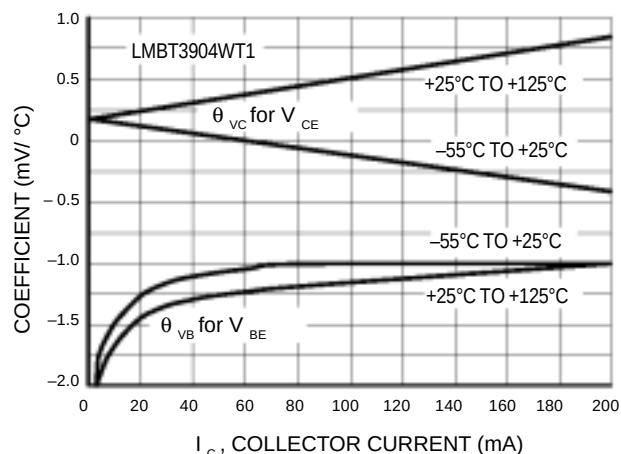
Figure 18. Temperature Coefficients
