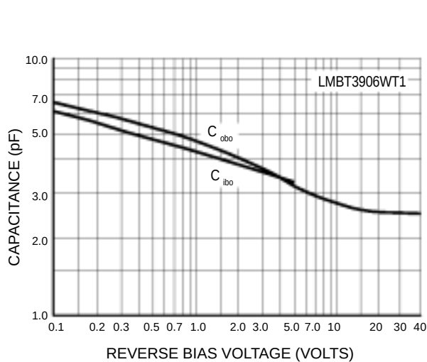
Figure 21. Capacitance
