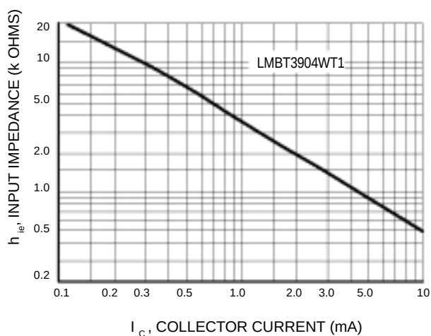
Figure 13. Input Impedance
