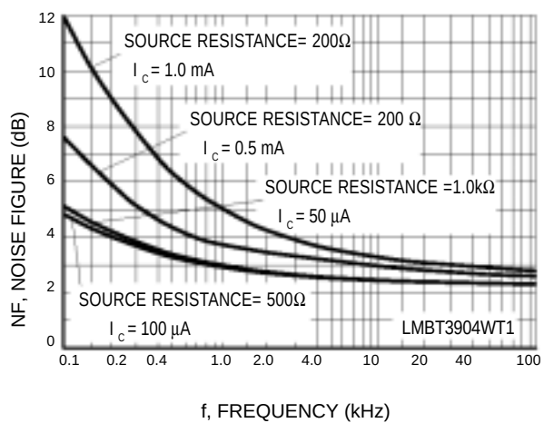
Figure 9. Noise Figure
