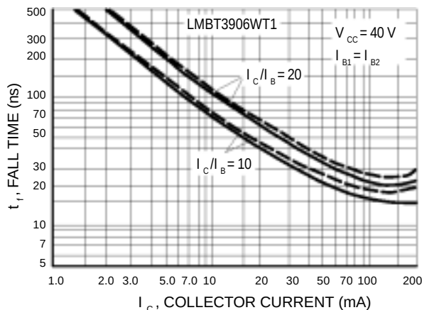
Figure 24. Fall Time
