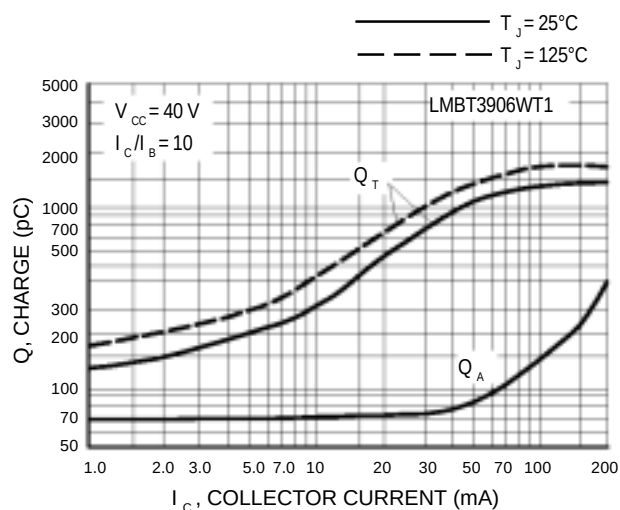
Figure 22. Charge Data
