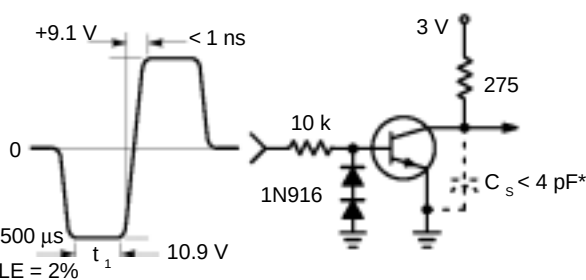
Figure 20. Storage and Fall Time Equivalent Test Circuit
