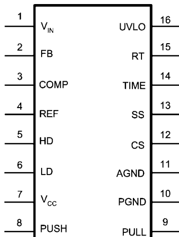
16-Lead TSSOP, LLP
