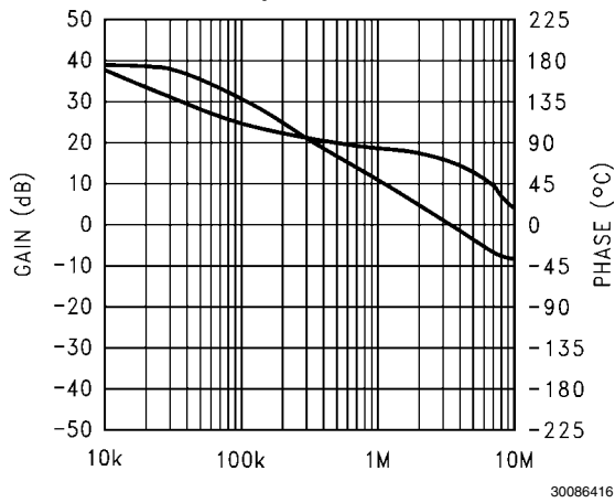
Error Amplifier Gain Phase
