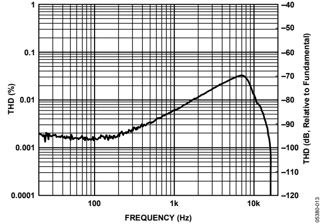
Figure 13. THD vs. Frequency, 1 W Output Power into 4 Ω Load, PVDD = 12 V
