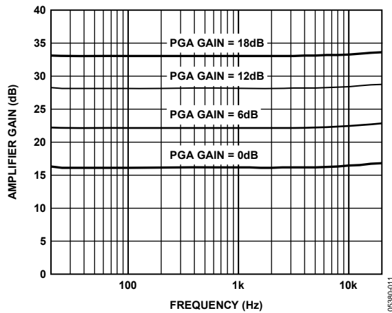
Figure 11. Amplifier Gain vs. Frequency, 6 Ω Load, PVDD = 12 V
