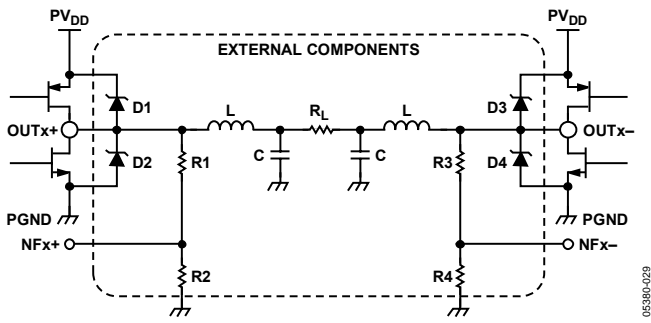
Figure 23. H-Bridge Configuration
