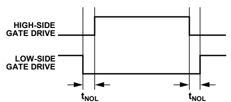
Figure 24. Half-Bridge Nonoverlap Delay Timing
