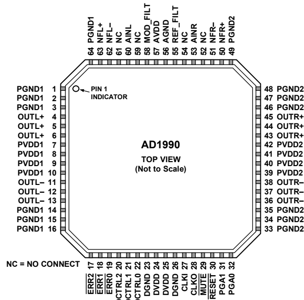
Figure 3. Pin Configuration
