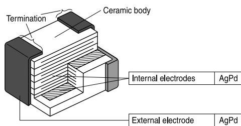
Multilayer varistor: Structure of silver-palladium termination
