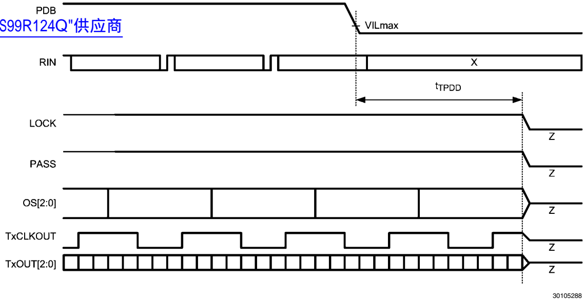
FIGURE 3. FPD-Link & LVCMOS Powerdown Delay
