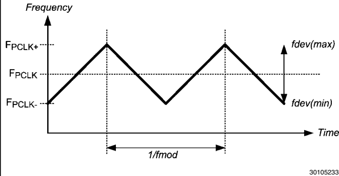
FIGURE 16. SSCG Waveform
