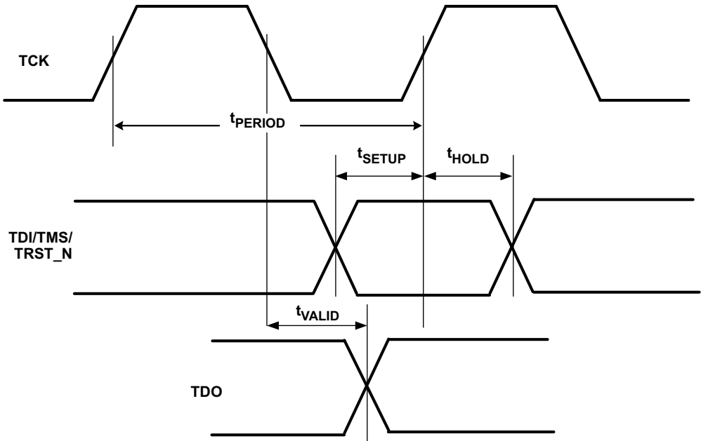
Figure 4-14. JTAG Timing
