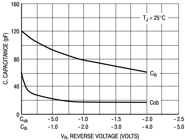
Figure 6. Capacitances
