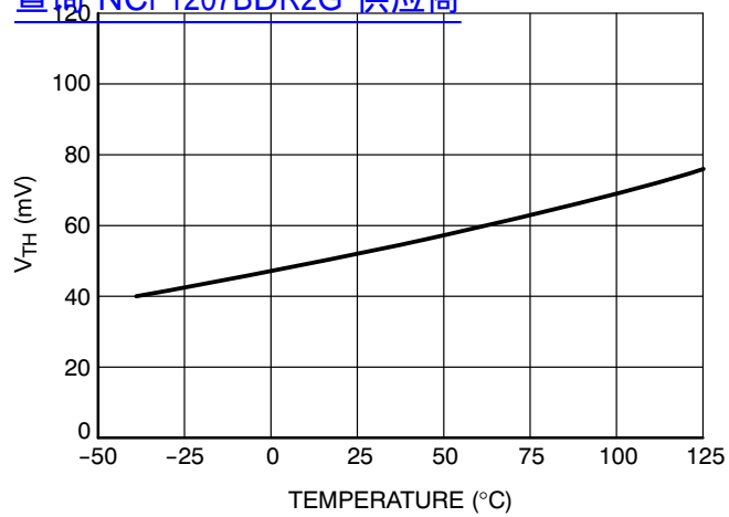
Figure 9. Input Voltage (Vpin1 Decreasing) versus Temperature
