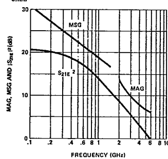
Figure 2. Typical MAG, Maximum Stable Gain (MSG) and |S_{21E}|^2 vs. Frequency (V CE = 18 V, I C = 30 mA), for the HXTR-5101.
