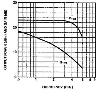
Figure 9. Typical P_{1dB} Linear Power and Associated 1 dB Compressed Gain vs. Frequency ( V_{CE} = 18 V, I_C = 30 mA), for the HXTR-5101.
