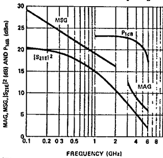
Figure 1. Typical MAG, Maximum Stable Gain (MSG), |S_{21E}|^2 and P 1dB Linear Power vs. Frequency (V CE = 18 V, I C = 30 mA), for the HXTR-5001.
