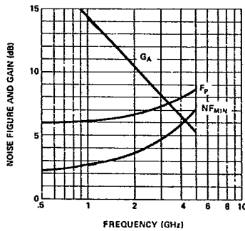
Figure 11. Typical Noise Figure NF_{MIN} and Associated Gain ( G_A ) When Tuned for Minimum Noise vs. Frequency ( V_{CE} = 18 V, I_C = 10 mA), Typical Noise Figure ( F_p ) When Tuned for Max P_{1dB} ( V_{CE} = 18 V, I_C = 30 mA), for the HXTR-5101 and HXTR-5103.
