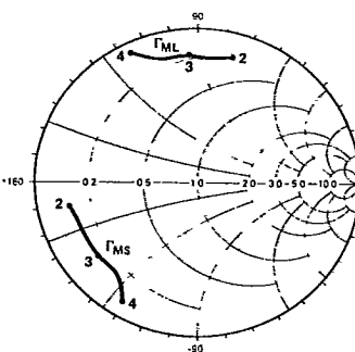
Figure 15. Typical \Gamma_{MS} , \Gamma_{ML} (Calculated From the Average S-Parameters) in the 2 to 4 GHz Frequency Range ( V_{CE} = 18 V, I_C = 30 mA), for the HXTR-5103.
