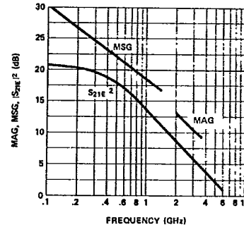
Figure 3. Typical MAG, Maximum Stable Gain (MSG), and |S_{21E}|^2 vs. Frequency (V CE = 18 V, I C = 30 mA), for the HXTR-5103.
