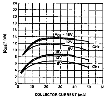
Figure 8. Typical |S_{21}|^2 vs. Collector Current at 1 and 2 GHz, for the HXTR-5103.
