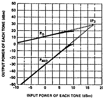
Figure 13. Typical Two Tone Third Order Intermodulation Distortion at 2 GHz for a Frequency Separation of 5 MHz ( V_{CE} = 18 V, I_C = 30 mA) for the HXTR-5103.
