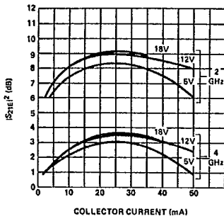
Figure 7. Typical |S_{21}|^2 vs. Collector Current at 2 and 4 GHz, for the HXTR-5101.
