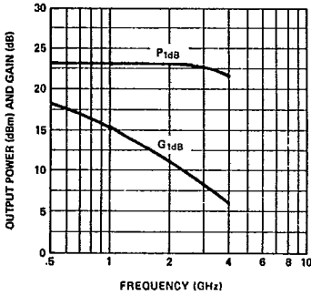
Figure 10. Typical P_{1dB} and Associated 1 dB Compressed Gain vs. Frequency ( V_{CE} = 18 V, I_C = 30 mA), for the HXTR-5103.
