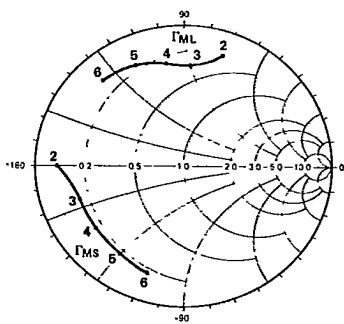
Figure 14. Typical \Gamma_{MS} , \Gamma_{ML} (Calculated From the Average S-Parameters) in the 2 to 6 GHz Frequency Range ( V_{CE} = 18 V, I_C = 30 mA), for the HXTR-5101.
