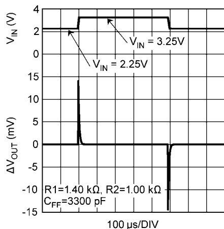
Line Transient V_{OUT} = 1.20V , C_{OUT} = 10\mu F Ceramic
