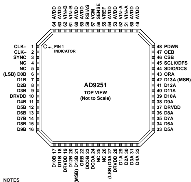
Figure 5. Pin Configuration
