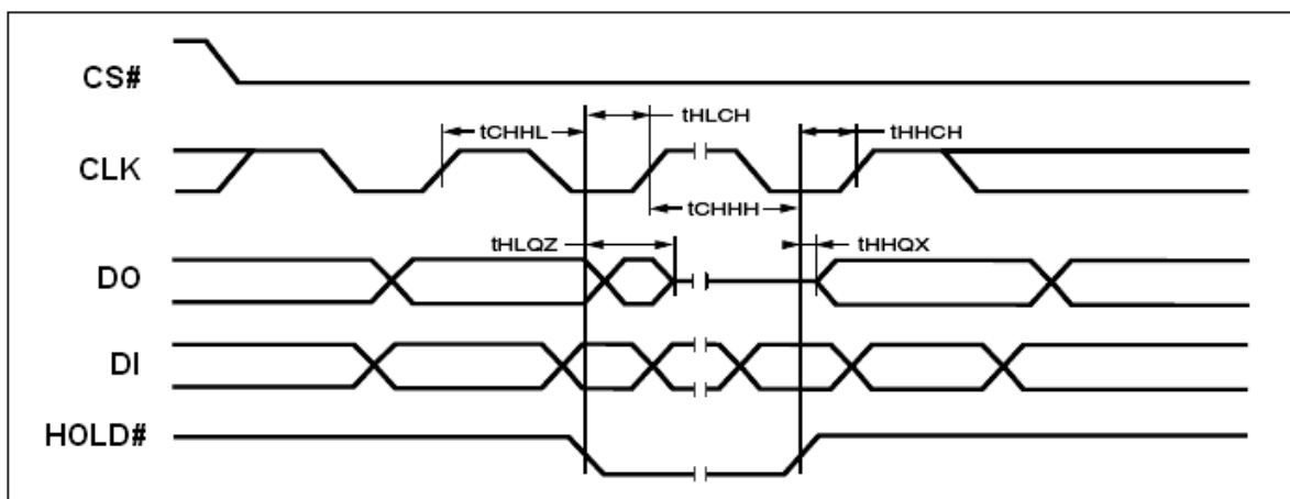
Figure 24. Hold Timing
