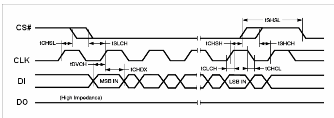
Figure 23. Input Timing
