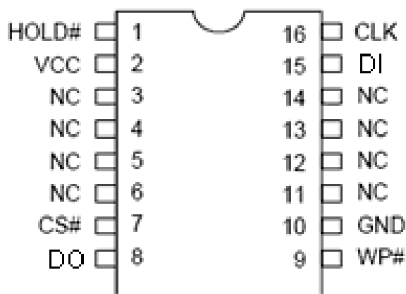
16 - LEAD SOP
