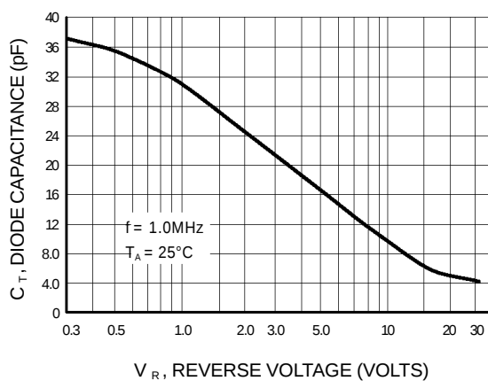
Figure 1. Diode Capacitance
