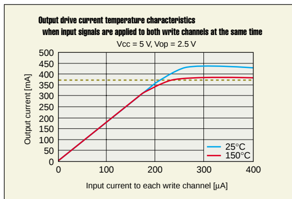
■ Figure 1 CD Output Drive Current Temperature Characteristics
