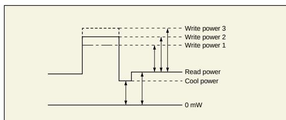
■ Figure 3 Sample 5-Value Recording Waveform
