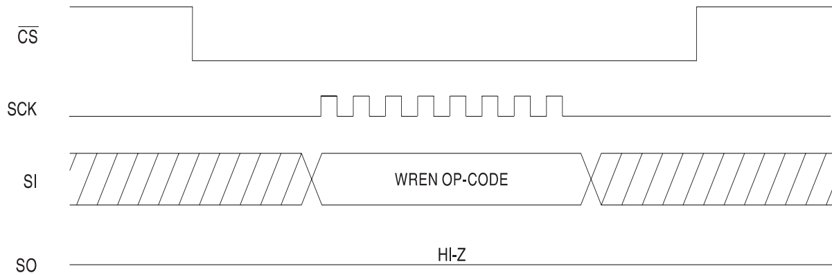
Figure 4. WREN Timing
