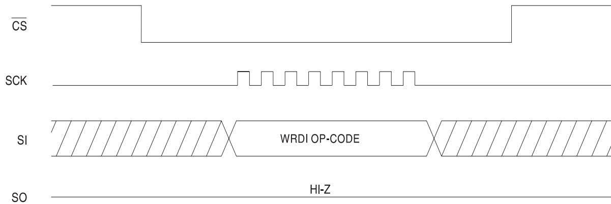
Figure 5. WRDI Timing
